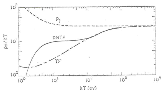
FIG. 4. Variation of pressure with temperature for iron at one-tenth normal density ( \rho = 0.785 g/cc).
