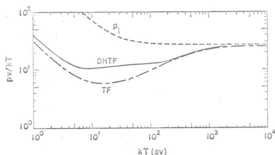
FIG. 3. Variation of pressure with temperature for iron at normal solid density ( \rho = 7.85 g/cc).
