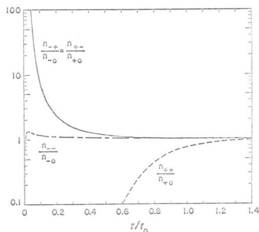
FIG. 6. The radial distribution functions for iron at normal density, \lambda = 1 , and kT = 1000 ev. The n_{--} curve lies above the n_{+-} curve for r/r_0 > 0.892 .
