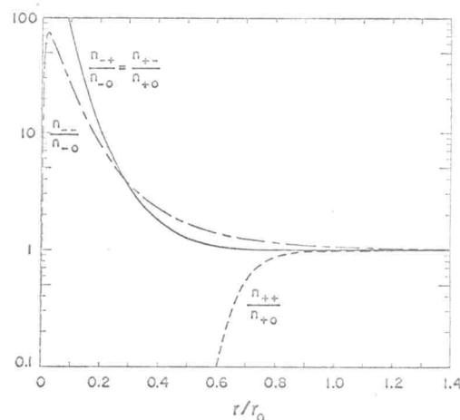
FIG. 5. The radial distribution functions for iron at normal density, \lambda = 1 , and kT = 100 ev.
